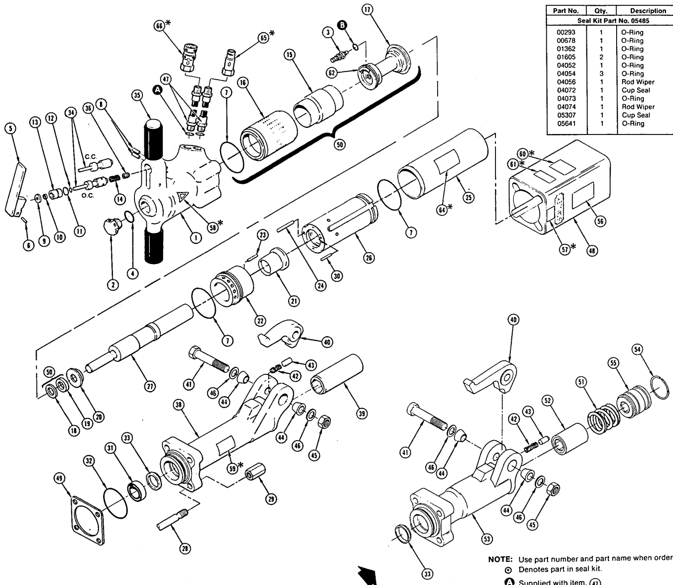
Easi-Ride™ Breaker Foot Assembly
